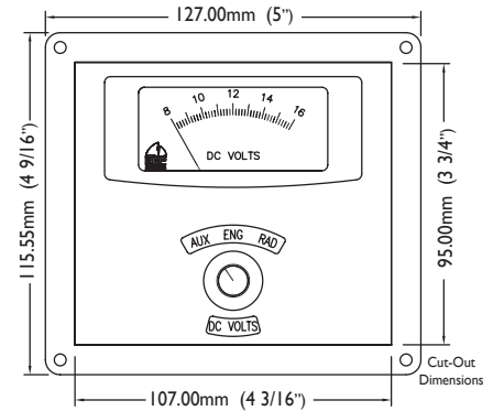
Dimensions for analog and digital panels
